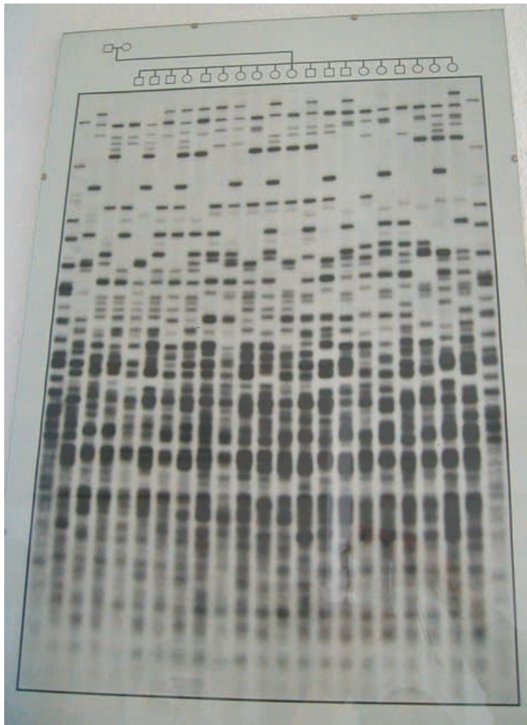
Fig. 1. Photo of a multi-plex gel on the wall of a DNA typing laboratory: RFLPs of variable, repetitive intronic region against the probe (CAC) 5 /(GTG) 5 (courtesy of Peter Nürnberg, Institute of Medical Genetics, Humboldt University, Berlin, Germany).
