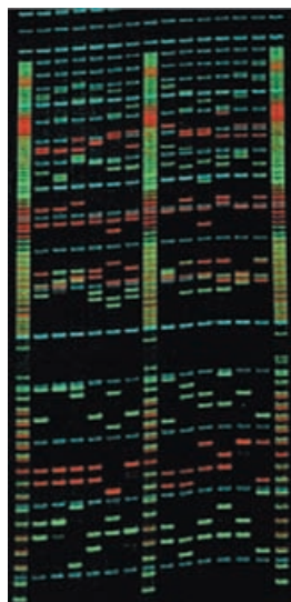
Fig. 3. A multiplex PCR of 16 short tandem repeat loci. The PCR products overlap and are therefore labelled in different fluorescent colours.
